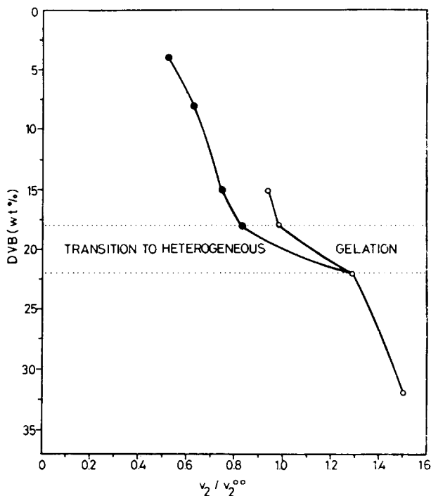
Fig. 7. Dependence of the swelling ratio, v_2/v_2^0 , on the DVB concentration for collapsed (●) and reexpanded (○) networks.
